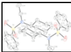
Fig. 1. The molecular structure of the title compound, with displacement ellipsoids at the 50% probability level. H atoms have been omitted for clarity.
